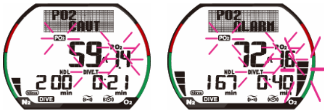
View 1 - PO2 limit warning with “PO2” and PO2 value blinking. View 2 - Exceeded PO2 with OLI graph blinking.
