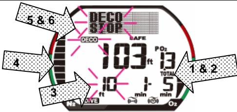
Decompression warning with “DECO STOP” and stop-depth information displayed
